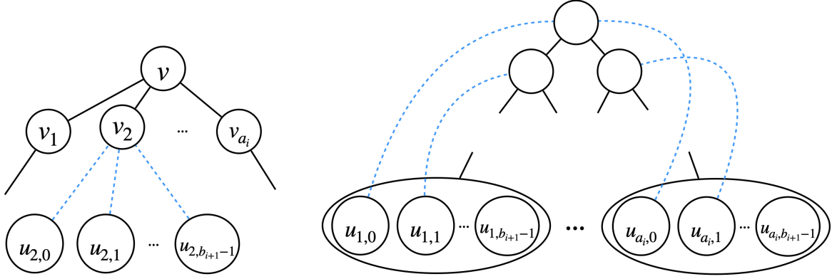
Figure 2: Left: The sub-tree rooted at a node v \in \mathcal{L}_k of depth i . The blue dashed edges represent that the u_{2,j} 's are leaves in the sub-tree rooted at v_2 . Right: The corresponding \mathcal{B}_v . The blue dashed edges correspond to edges in the bipartite graph G .
