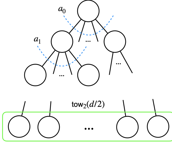
Figure 1: The tree \mathcal{L}_k . The vertices in the green box are identified as the left vertices of the bipartite graph G , while those outside the box correspond to the right vertices.
